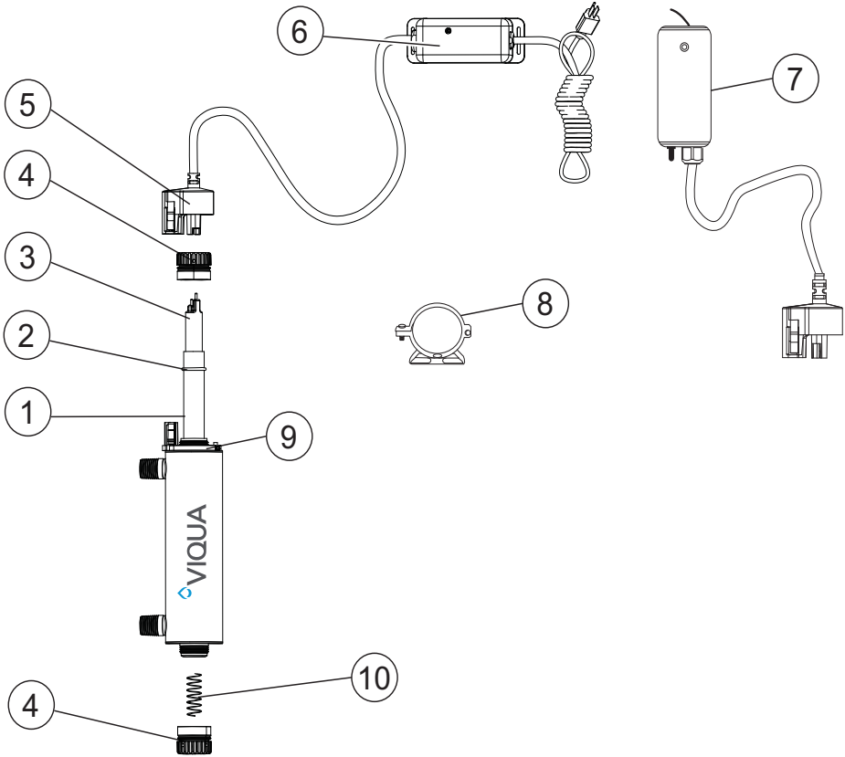
Figure 1 System Components
