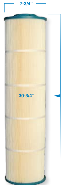
Hurricane® Cartridge Length and O.D.
