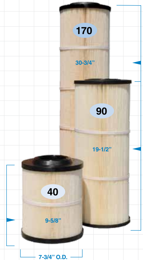
Hurricane® Cartridges
