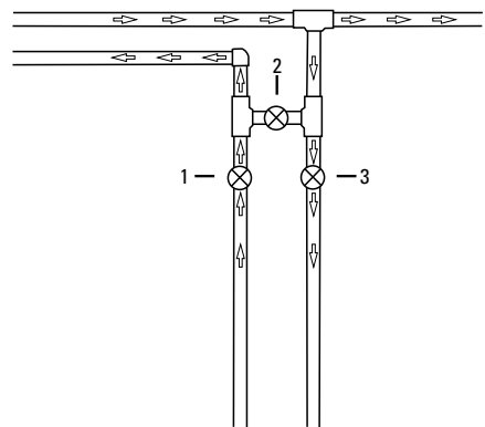
Figure 9 Manual Bypass
